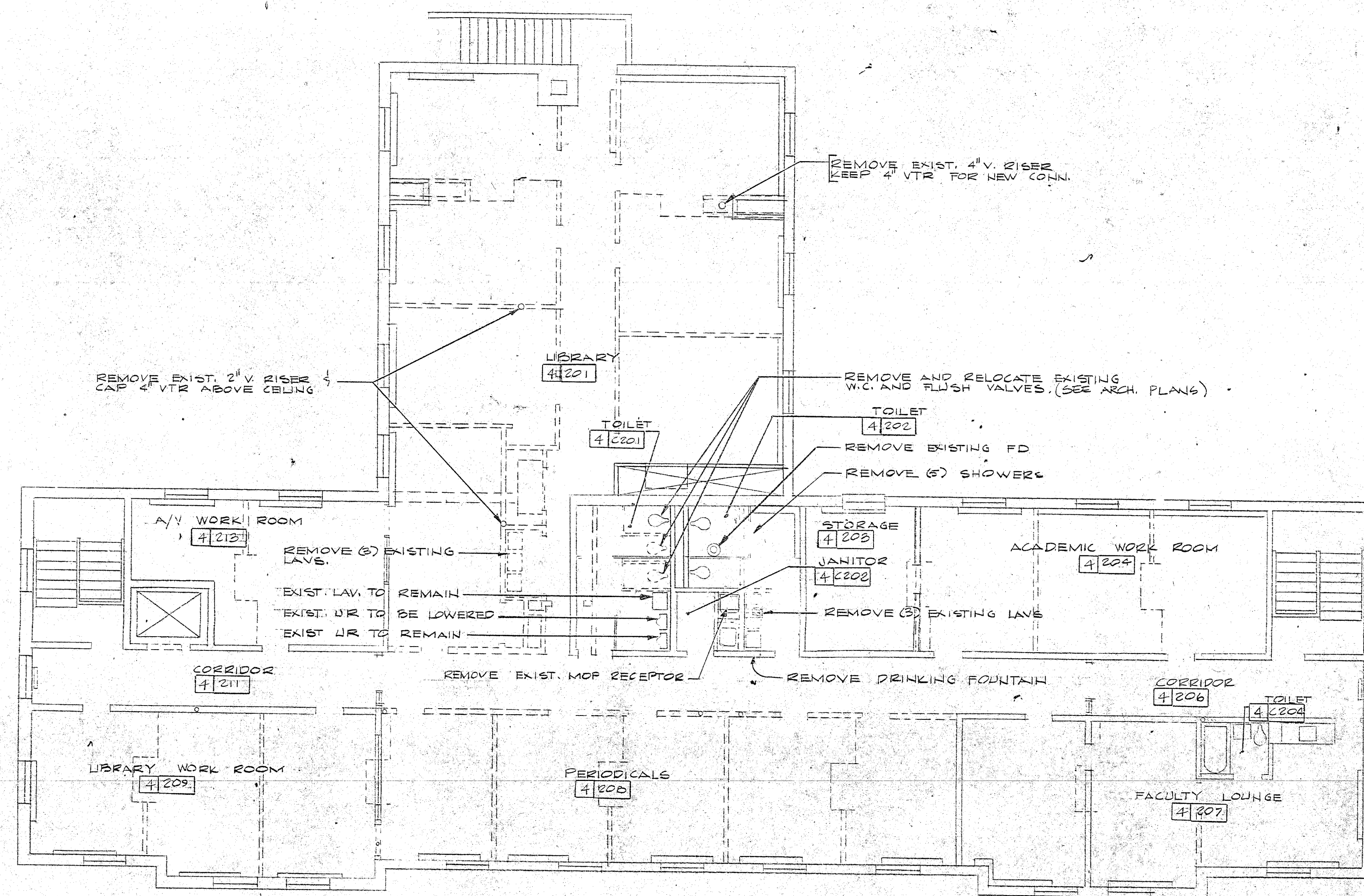
RENOVATION WORK SECOND FLOOR PLAN
