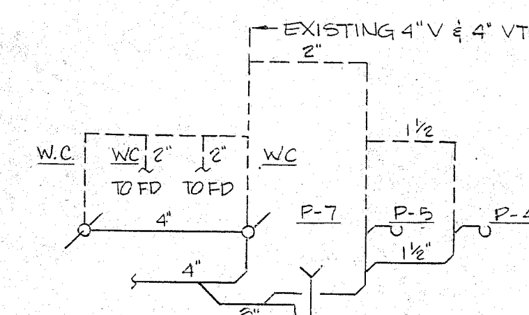
SANITARY RISER "A" NO SCALE
