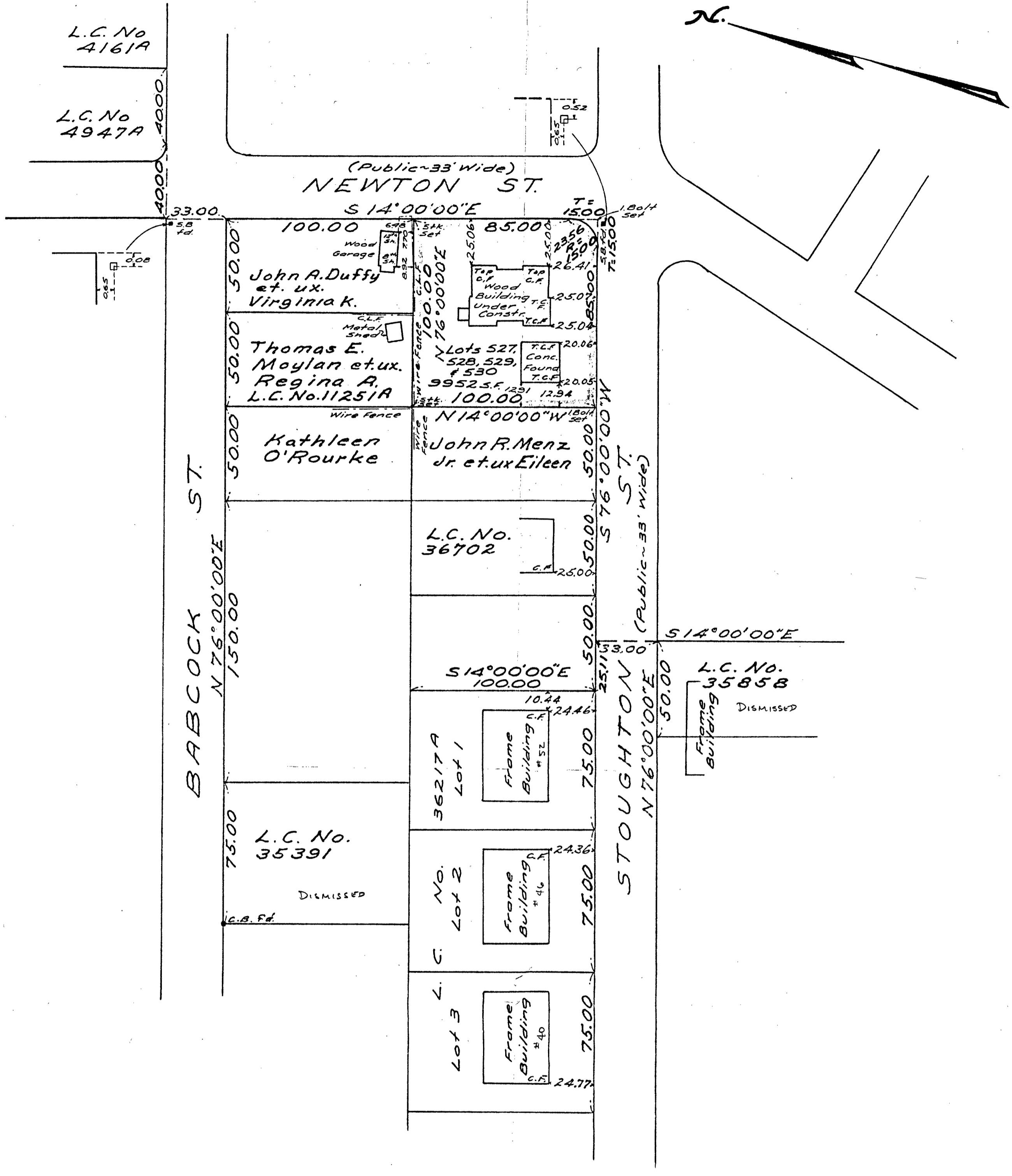
Plan of Land in Quincy, Mass. Scale 40 feet to an inch Jan. 13, 1984 Ernest W. Branch Inc., Civil Engineers Munroe Building, 1245 Hancock St., Quincy
