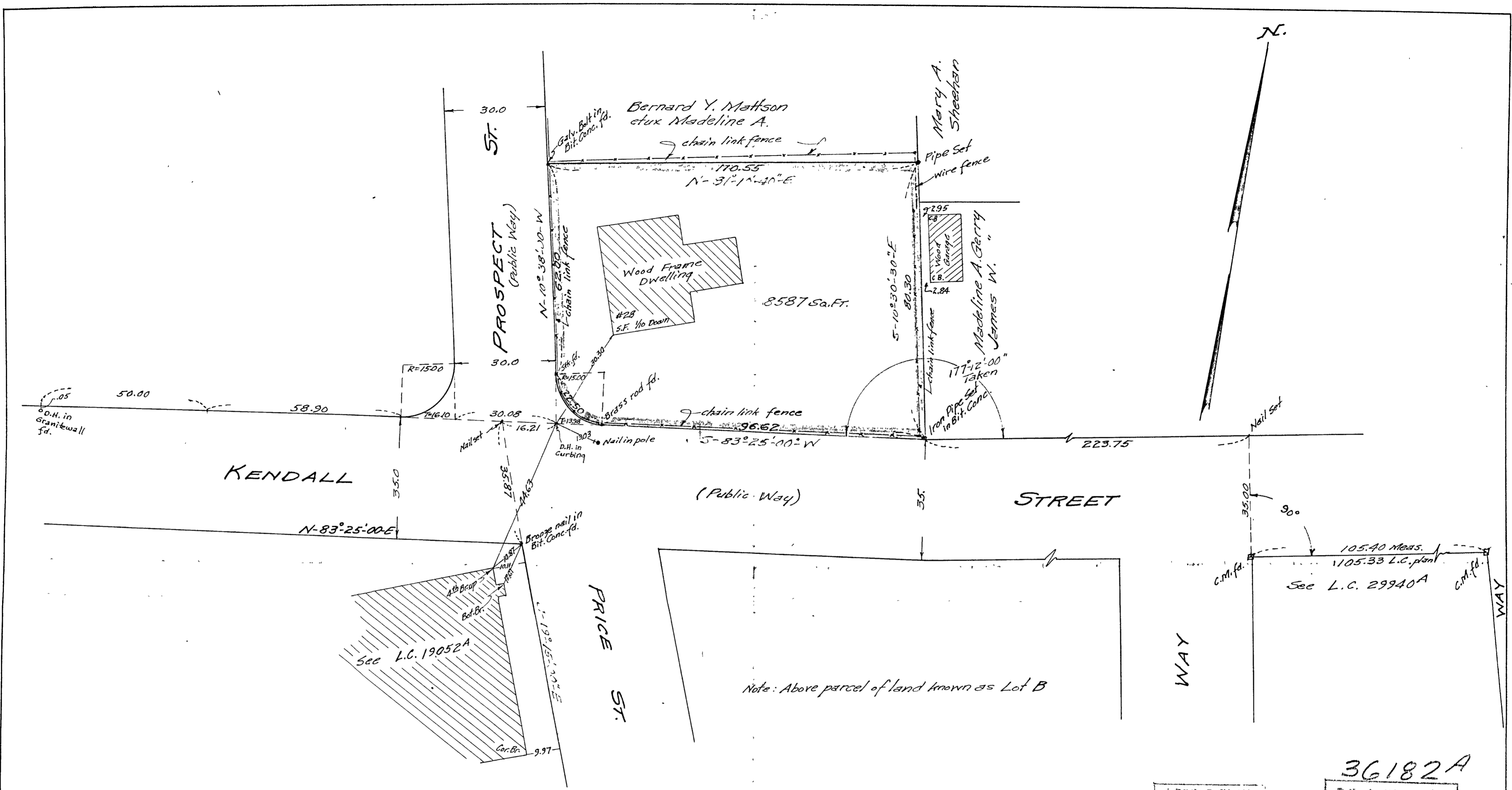
PLAN OF LAND IN QUINCY SCALE: 1"=20' APRIL 1969 GEORGE BAROUD R.L.S. 24 CHASE ST. QUINCY-MASS.
