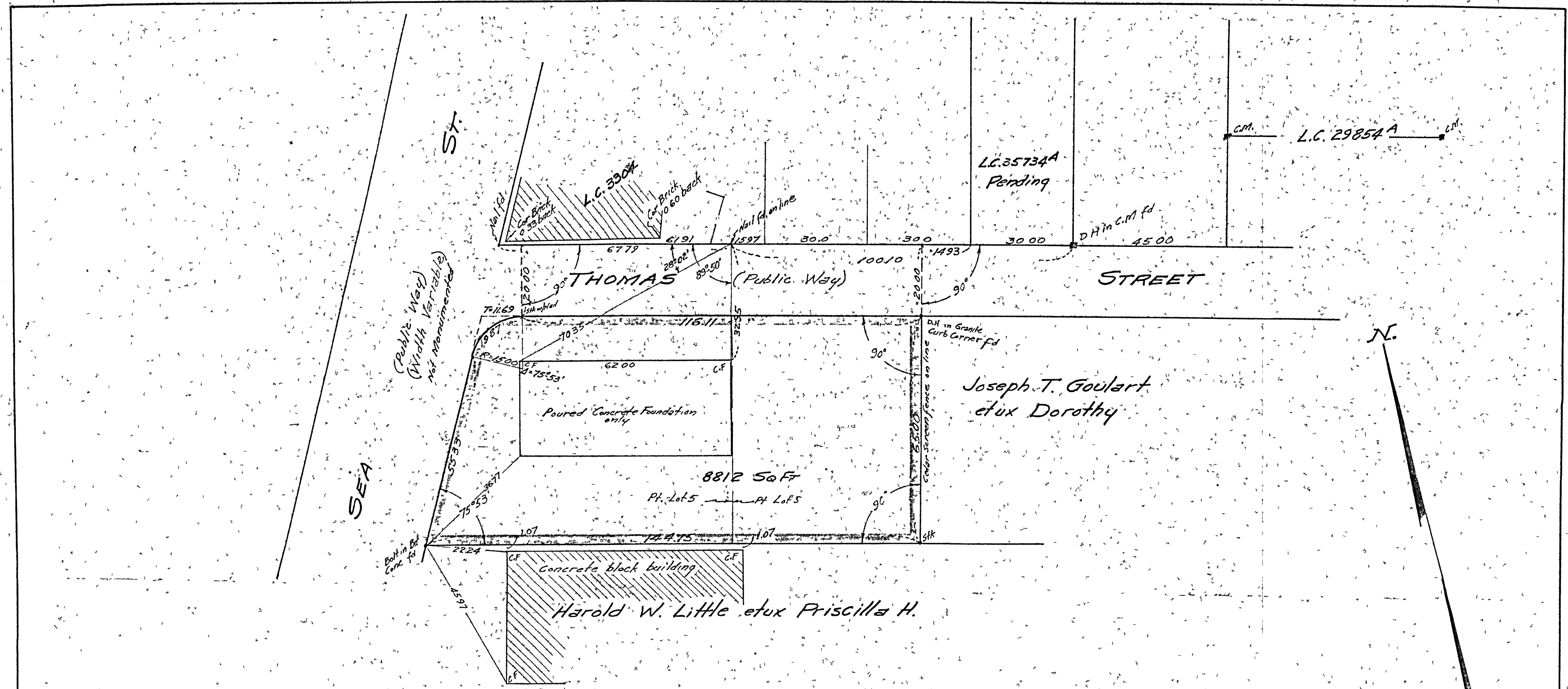
PLAN OF LAND IN QUINCY SCALE: 1"=20' JANUARY 11, 1969 GEORGE BAROUD-R.L.S.
