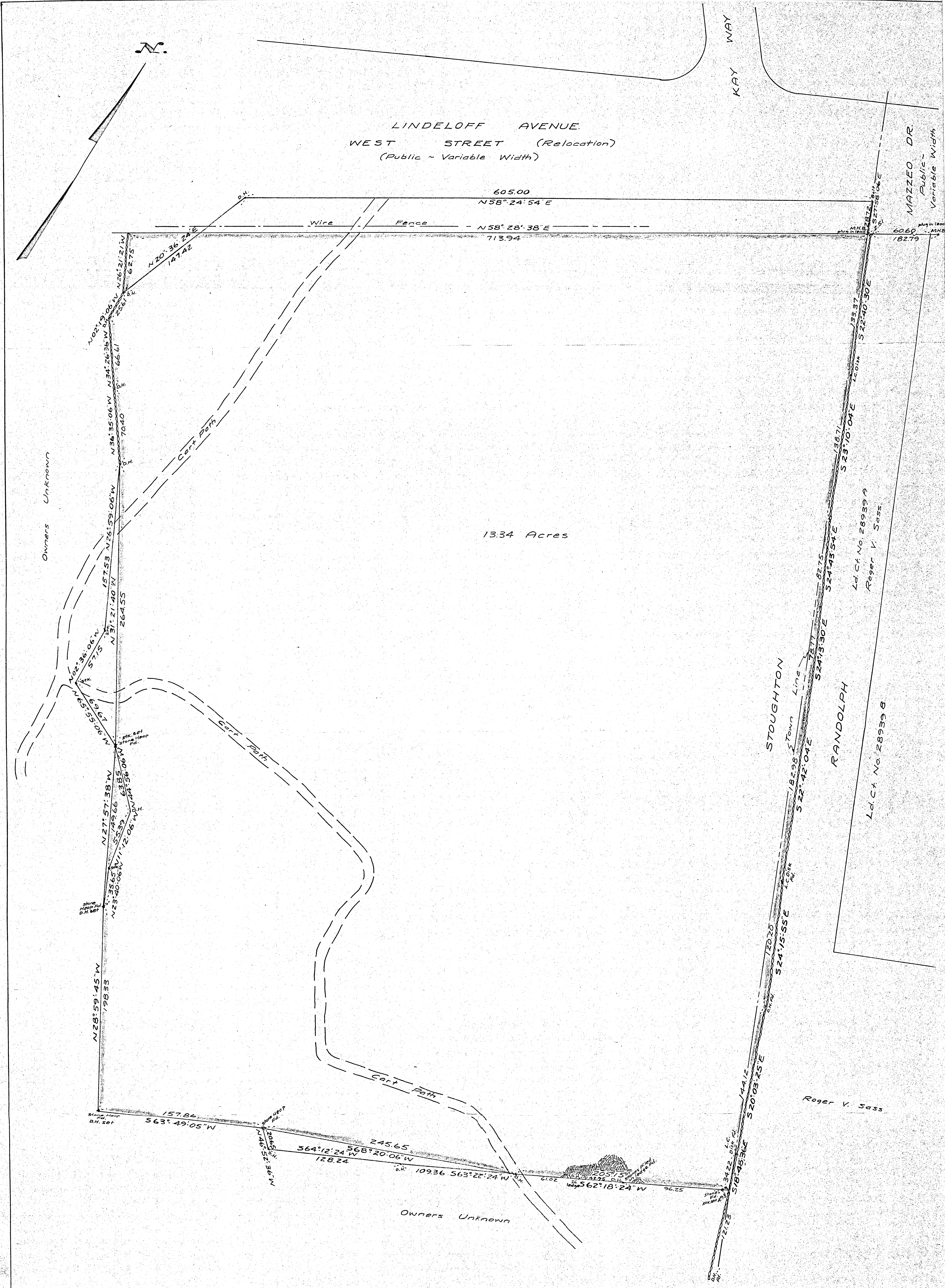
Plan of Land in Stoughton, Mass. Scale 40 feet to an inch September 21, 1968 Ernest W. Branch Inc., Civil Engineers Adams Building, 1354 Hancock St., Quincy
