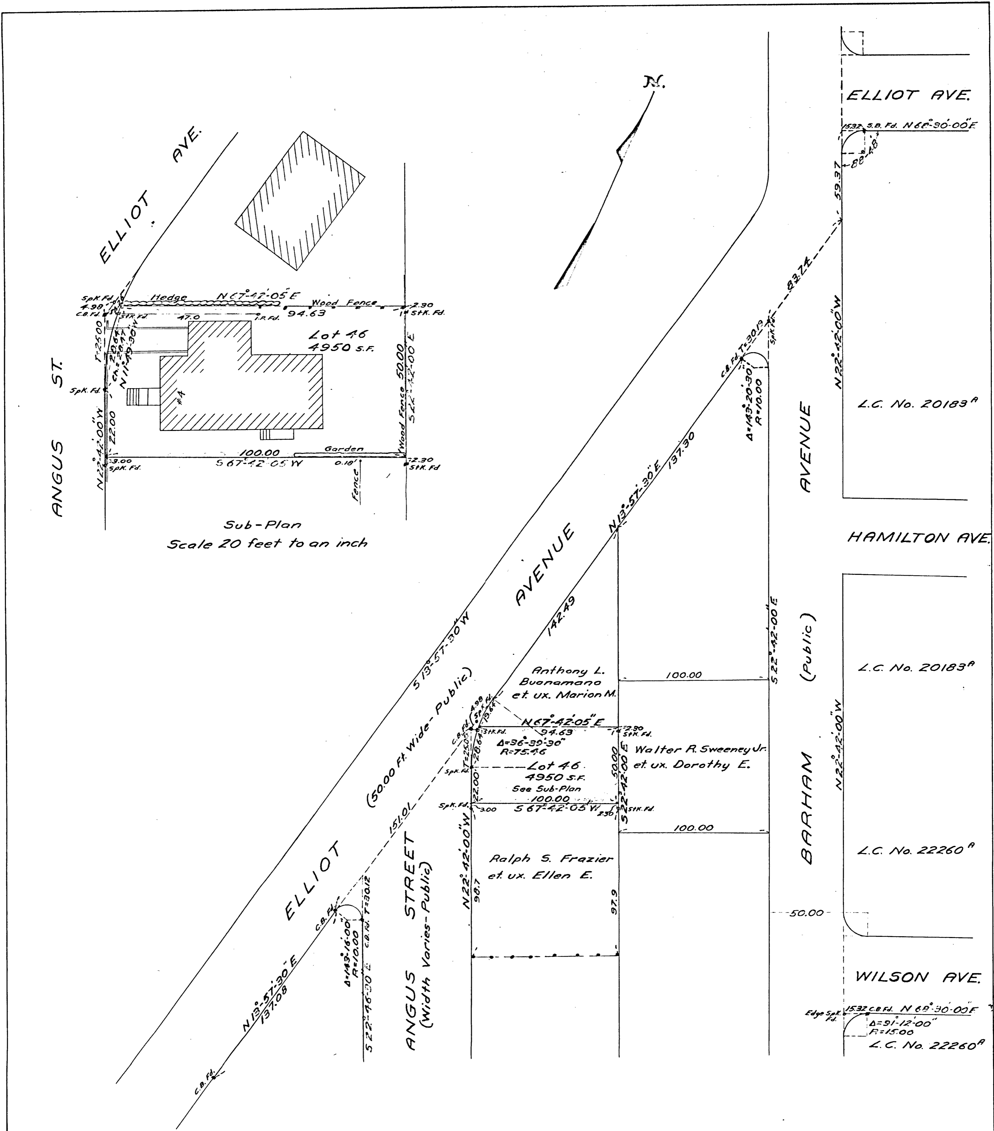
Plan of Land in Quincy, Mass. Scale 40 feet to an inch April 14, 1964 Ernest W. Branch Inc., Civil Engineers 11 Adams Building, Quincy
