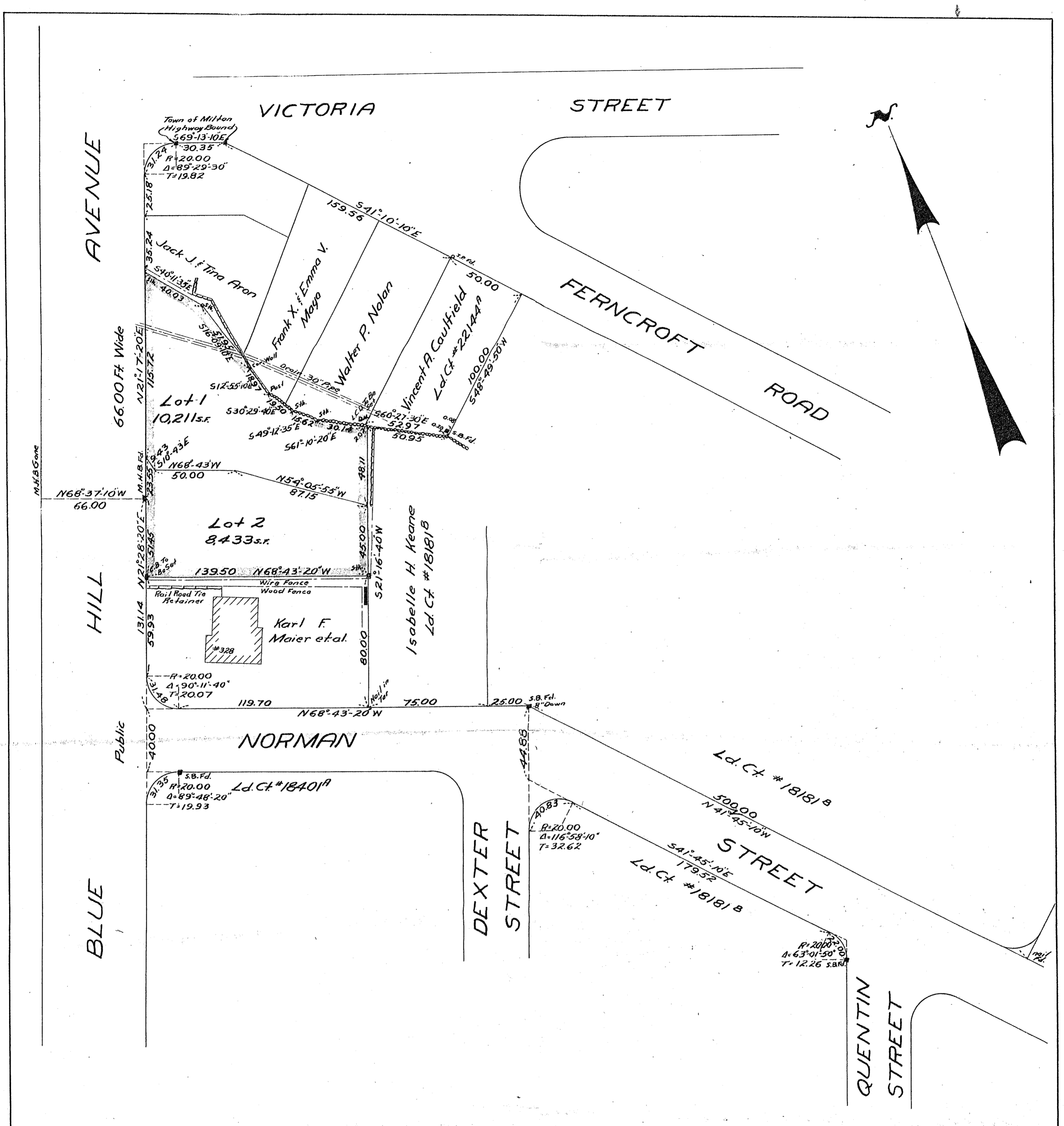
Plan of Land in Milton, Mass. Scale 40 feet to an inch April 5, 1963 Ernest W. Branch Inc., Civil Engineers 11 Adams Building, Quincy
