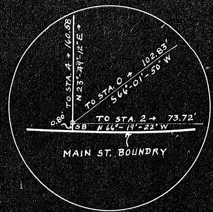
DETAIL OF STA 3 NOT TO SCALE
