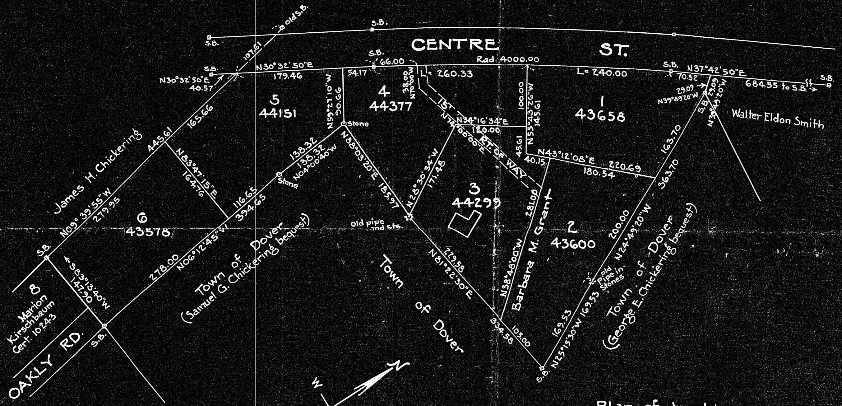
Plan of Land in DOVER, MASS. Scale 1 in. = 100 ft. E.W. Pilling Engineer Jan. 14, 1941
