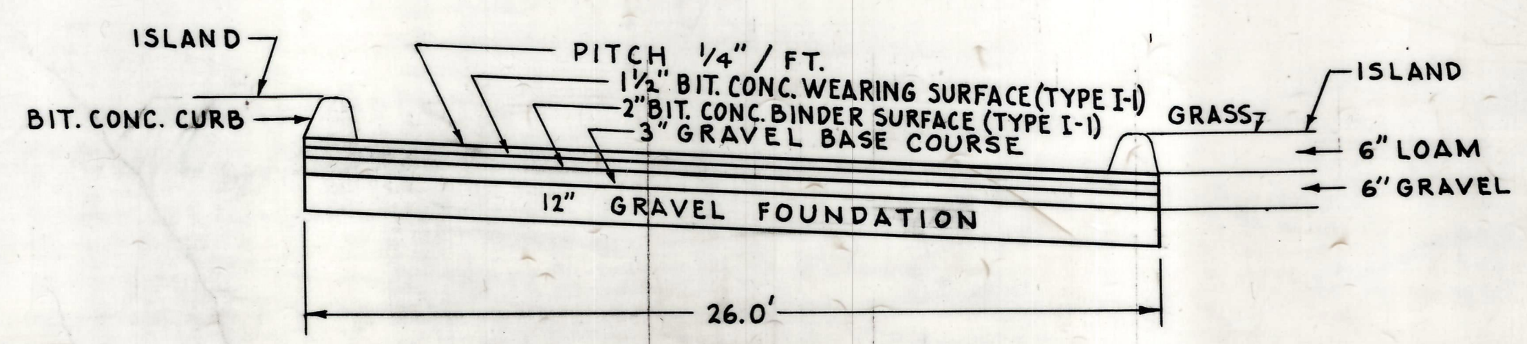
COMMON STREET - TYPICAL SECTION Not to Scale
