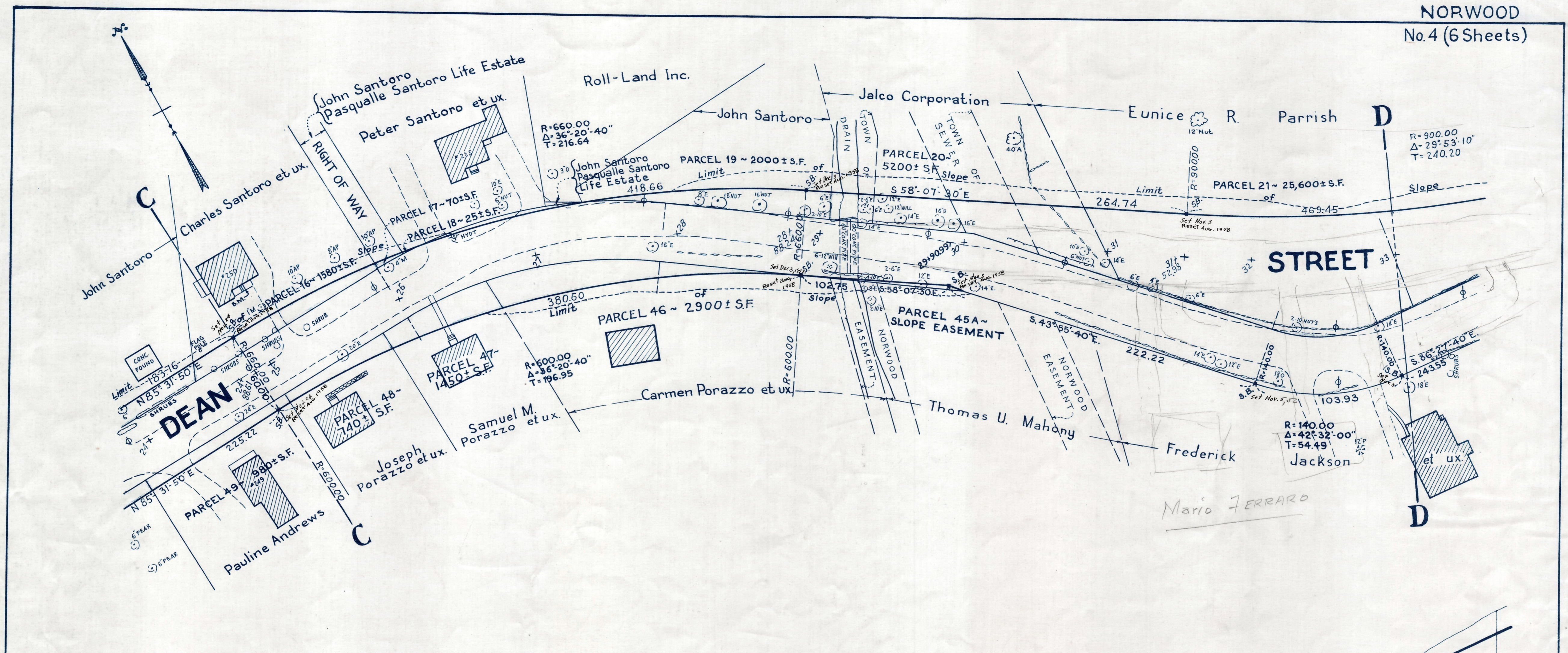
REVISED PROFILE STA. 23+00 to STA 31+45 JANUARY 1958
