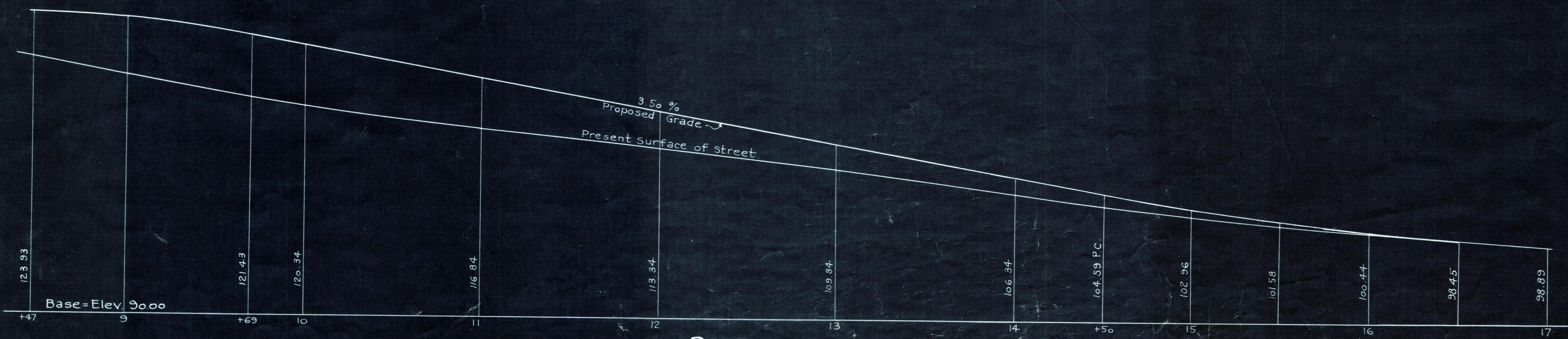
PROFILE Hor. Scale 1 inch = 40 feet Vert. " 1 " = 8 "
