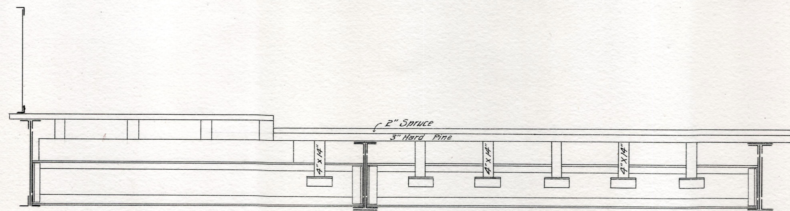
Half Section showing Girders Scale \frac{1}{2} Inch = 1 Foot
