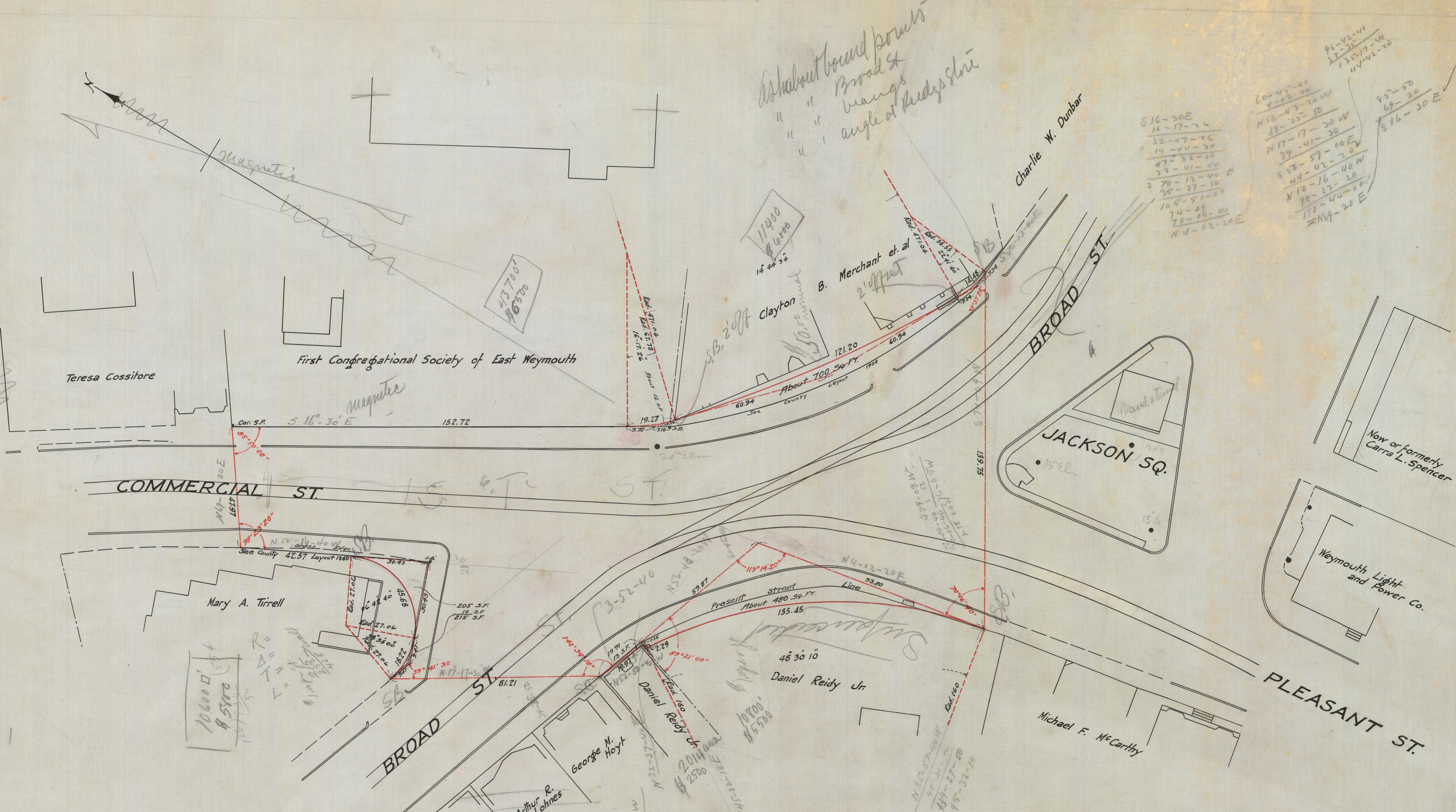
PLAN SHOWING PROPOSED WIDENING AT OR NEAR JACKSON SQUARE EAST WEYMOUTH, MASS. SCALE: 1 INCH = 20 FEET JANUARY 22, 1925 RUSSELL H. WHITING, CIVIL ENGINEER NORTH WEYMOUTH, MASS.
