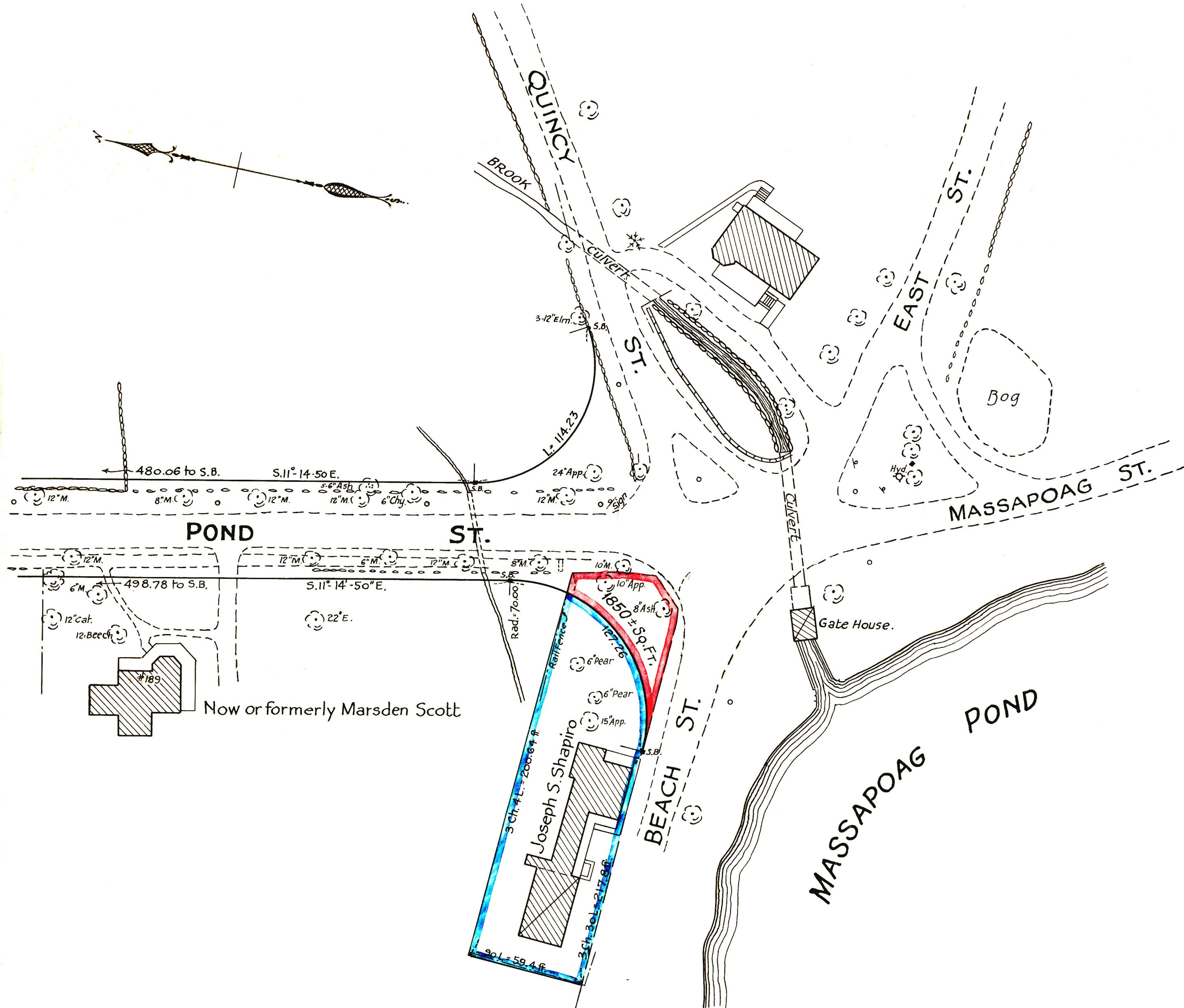
Plan showing Taking by Norfolk County Commissioners by Return dated May 1, 1928, at the Corner of Pond and Beach Streets. Scale 1 in. = 40 ft. May 12, 1937. Hartley L. Wite, County Engineer.
